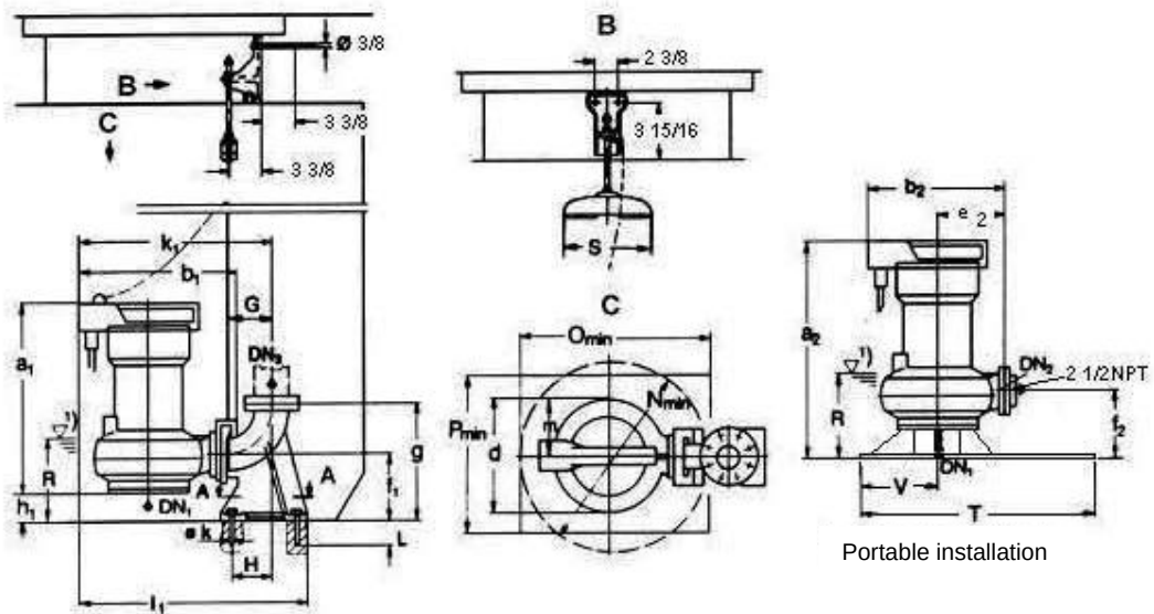
Stationary installation
