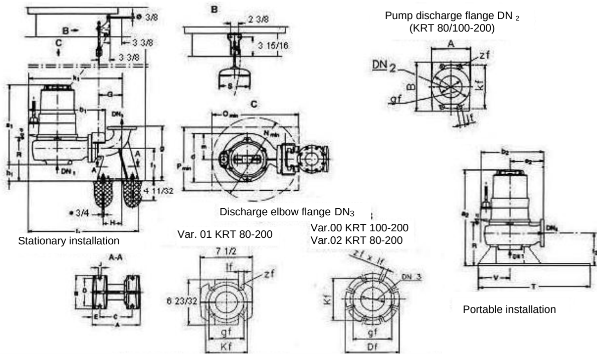
DISCHARGE ELBOW FOUNDATION
